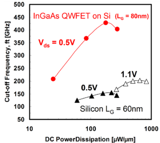
Fig. 12: Cut-off frequency as a function of DC power dissipation for the e-mode L_G=80\text{nm} \text{In}_{0.7}\text{Ga}_{0.3}\text{As} QWFET on Si at V_{DS}=0.5\text{V} , versus standard Si n-MOSFET transistor with L_G=60\text{nm} at V_{DS}=0.5\text{V} and 1.1\text{V} .
