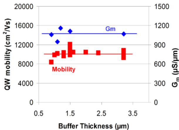
Fig. 11: QW mobility and transconductance ( G_m ) as a function of composite buffer layer thickness.
